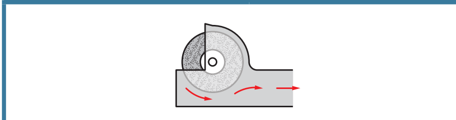
DIAGRAM 3: Enclosure around a grinding wheel
