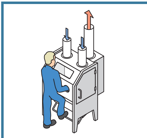
DIAGRAM 1: Abrasive blasting cabinet
