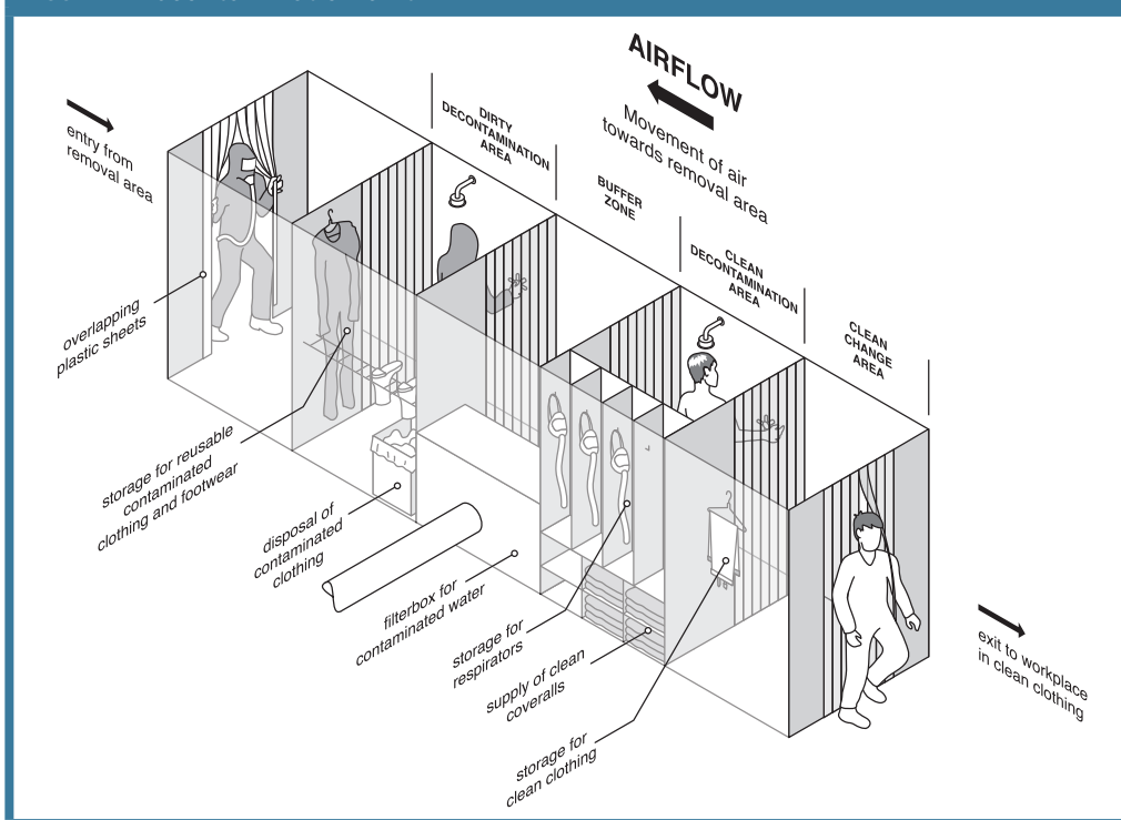
FIGURE 1: Decontamination unit.
