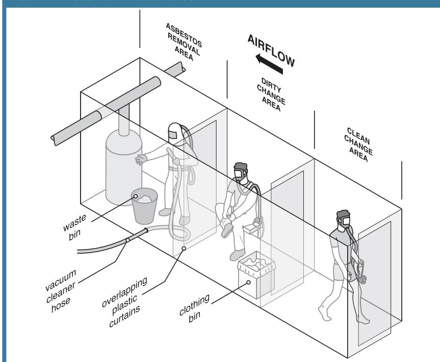
FIGURE 2: Decontamination area.
