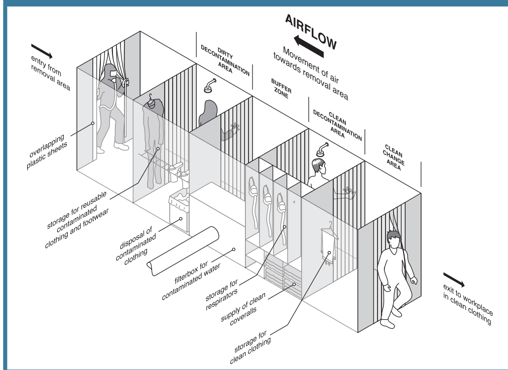
FIGURE 1: Decontamination unit.
