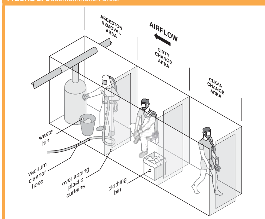
FIGURE 2: Decontamination area.
