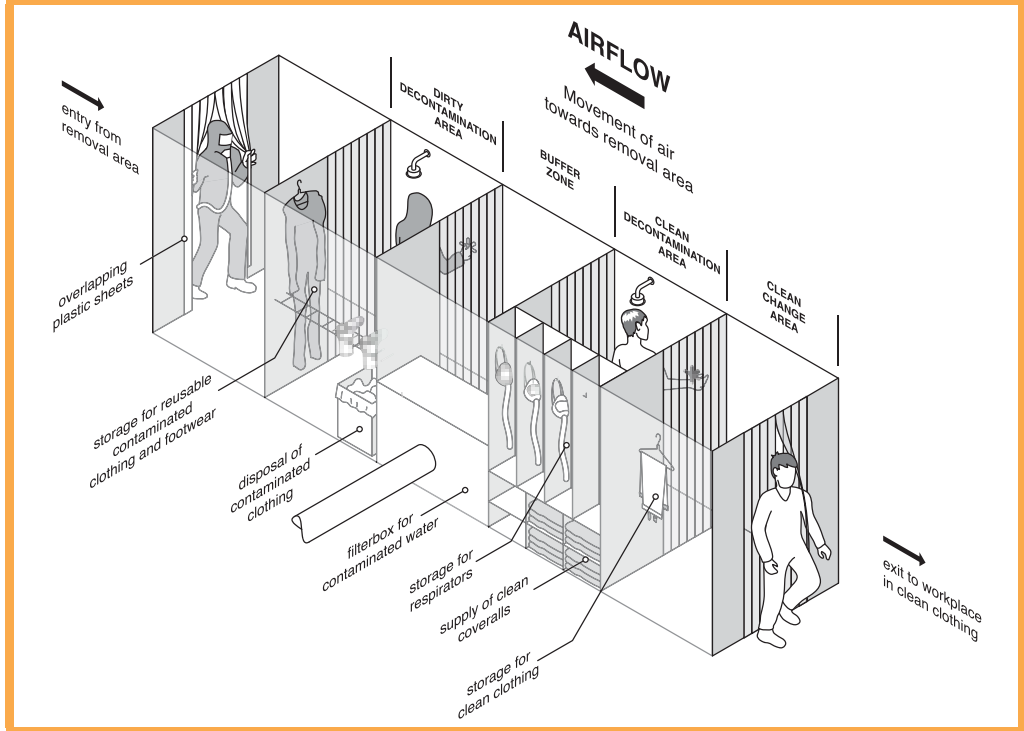
FIGURE 1: Decontamination unit.
