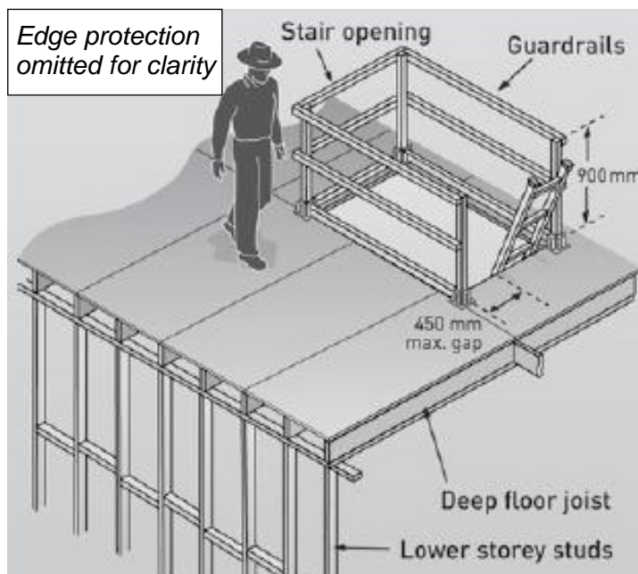
Figure 13: Void at upper level guarded
