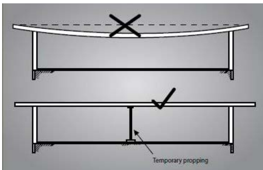
Figure 15: Method of supporting long trusses
