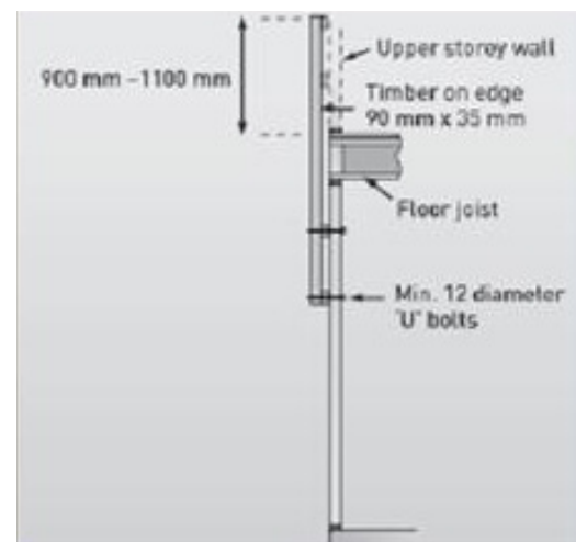
Figure 11: Examples of upper floor edge protection
