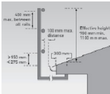
(c) Guardrail outside roof line (Note: If gutter not present, then the 100mm maximum distance is measured from the fascia board or outer ends of the rafters or top chords to trusses)
