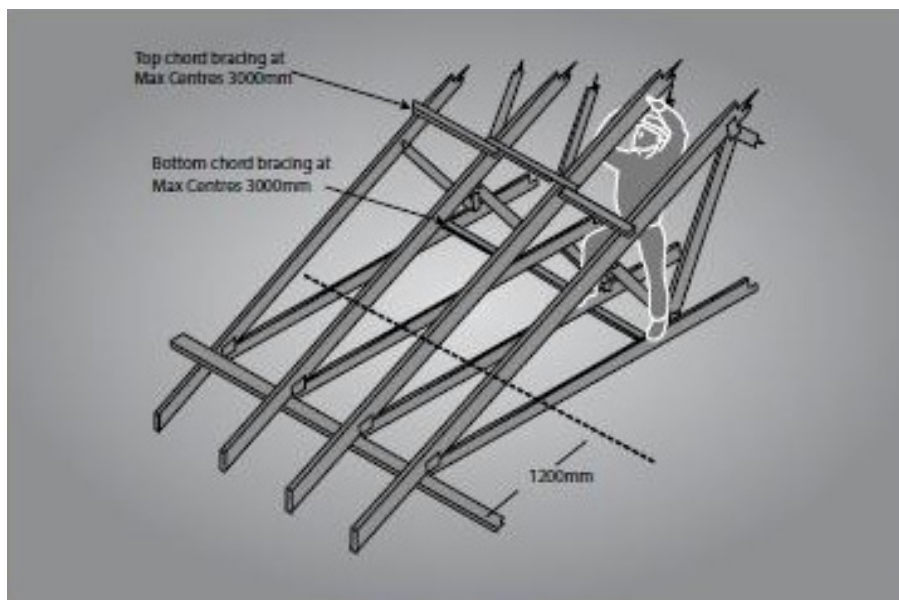
Figure 16: ‘No go’ zone for persons erecting trusses
