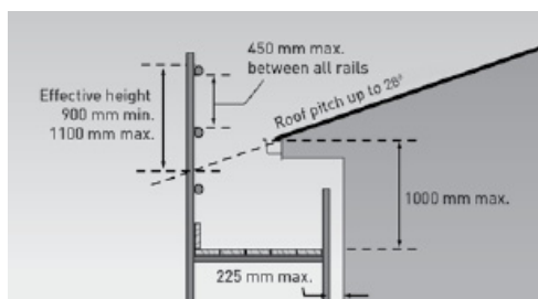
(a) Roof pitch up to 26°
