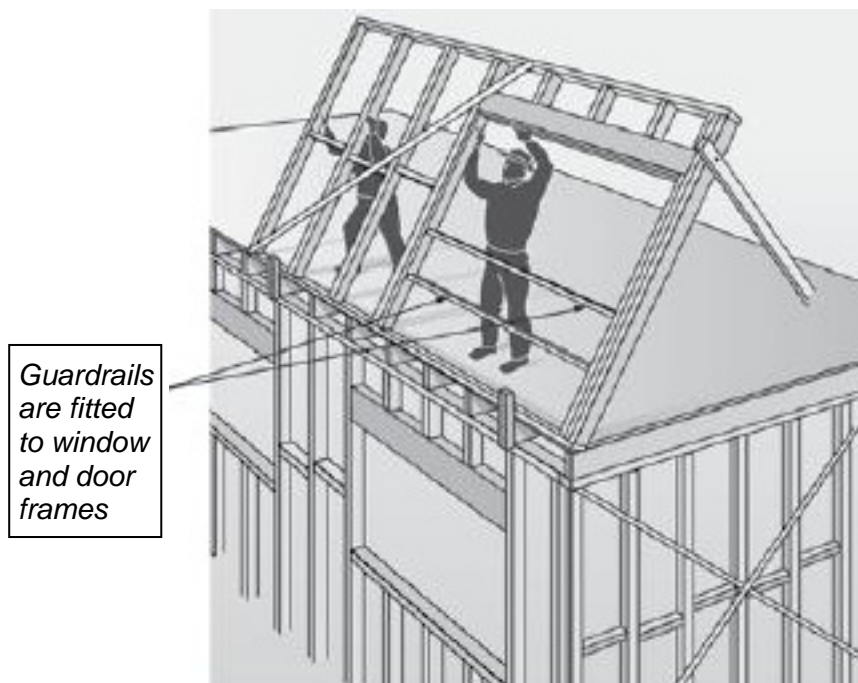
Figure 14: Erecting upper level wall frames
