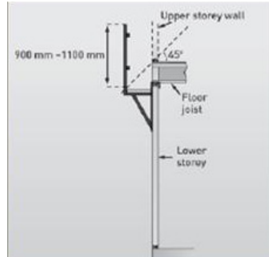
Figure 10: Examples of upper floor edge protection
