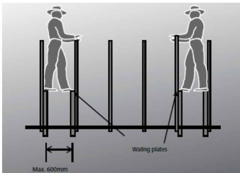
Figure 18: Showing the positions for pairs of waling plates
