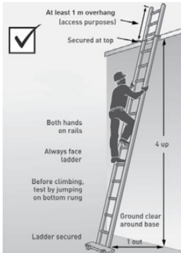
Figure 8: Example of acceptable ladder use
