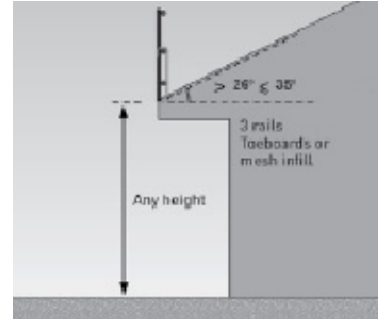
(b) Roof pitch greater than 26°
