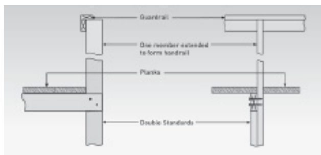
Detail 'A' Putlog to standard
