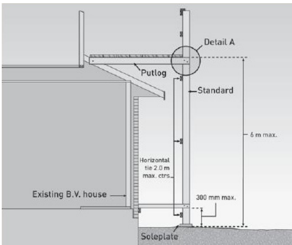
Figure 26: Timber scaffold (single pole – high first lift)
