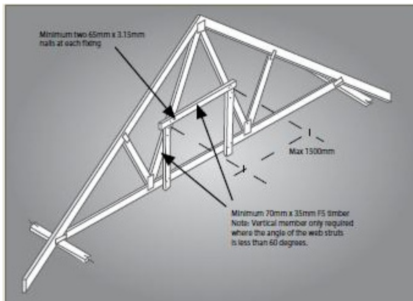
Figure 17: Suggested method of fixing temporary waling plate
