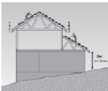
(e) Installing roofing at two levels (Note: end guardrails omitted for clarity)
