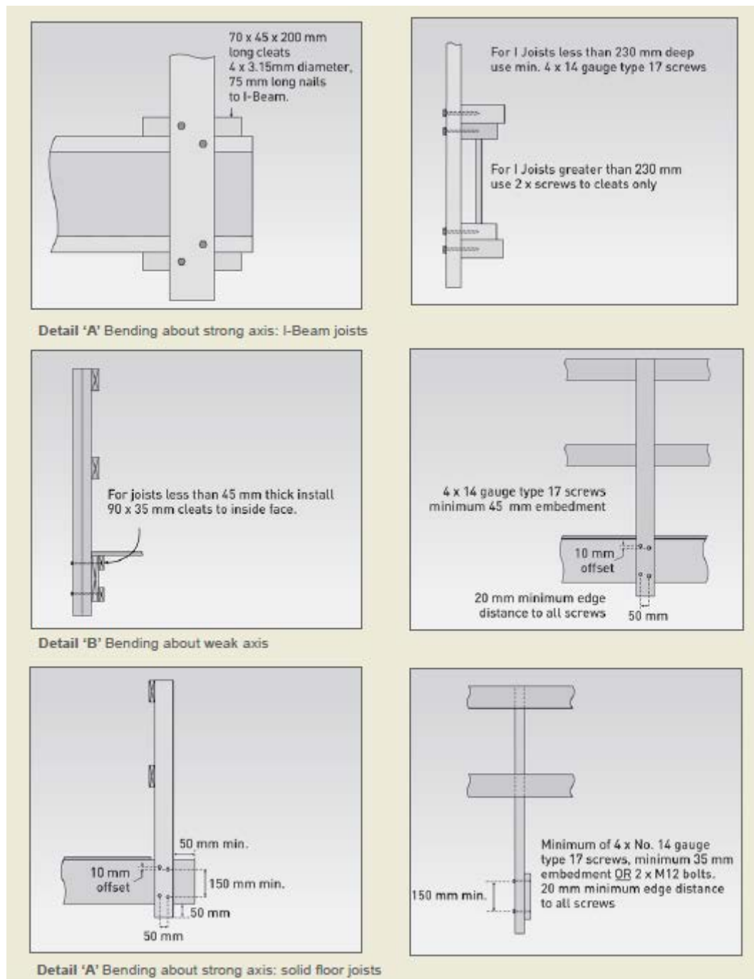
Figure 4: Timber guardrails
