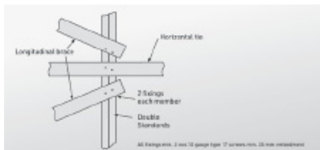
Bracing details
