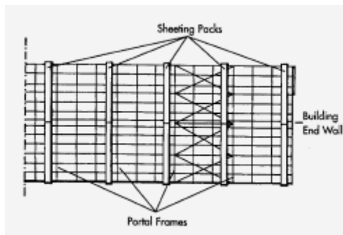
Figure A15. Location of sheeting packs.
