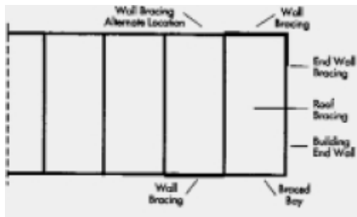
Figure A3. Building wall bracing location
