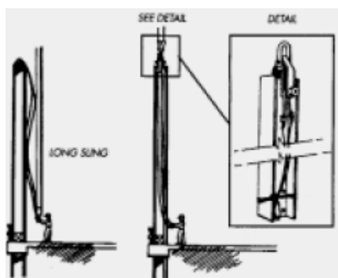
Figure 5. Remote release shackles
