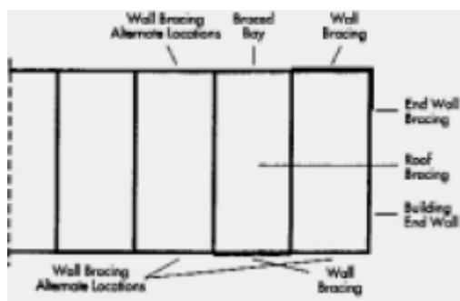
Figure A1. Building bracing location – internal bay
